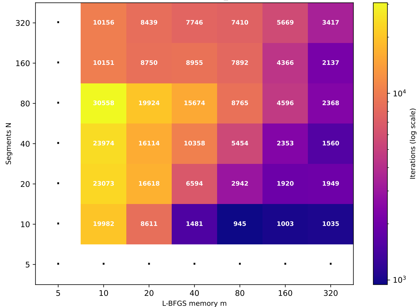
Recurrence T \approx 41.36 (target T=40 , rec_id=24) [36/49 converged]
