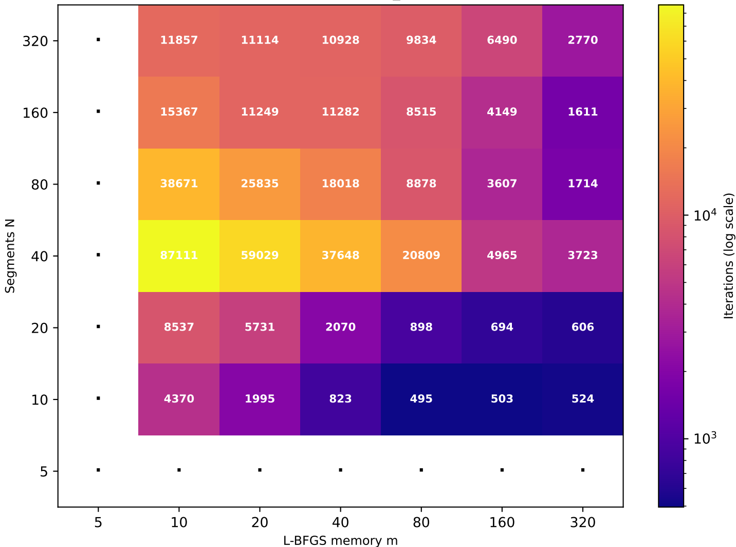
Recurrence T \approx 38.33 (target T=40 , rec_id=25) [36/49 converged]
