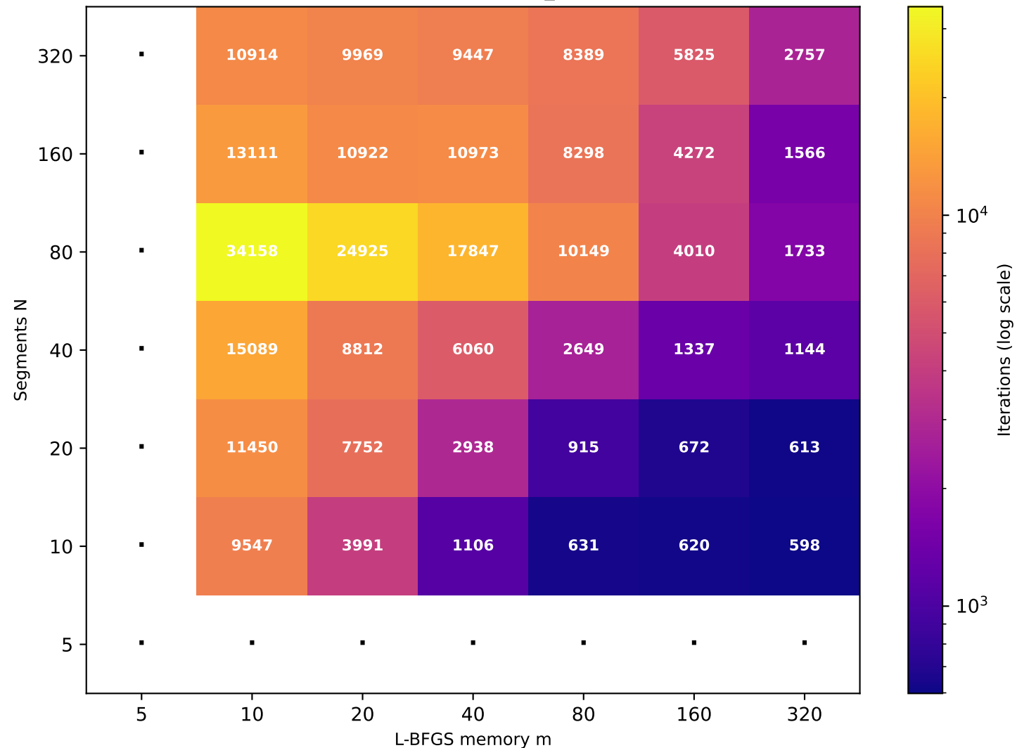
Recurrence T \approx 39.96 (target T=40 , rec_id=26) [36/49 converged]
