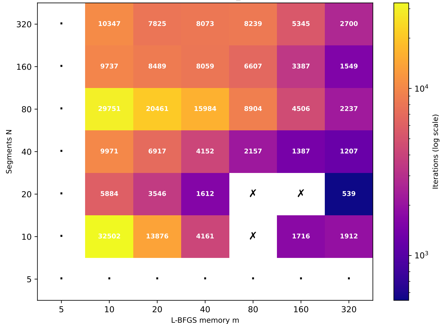
Recurrence T \approx 37.90 (target T=40 , rec_id=28) [33/49 converged]
