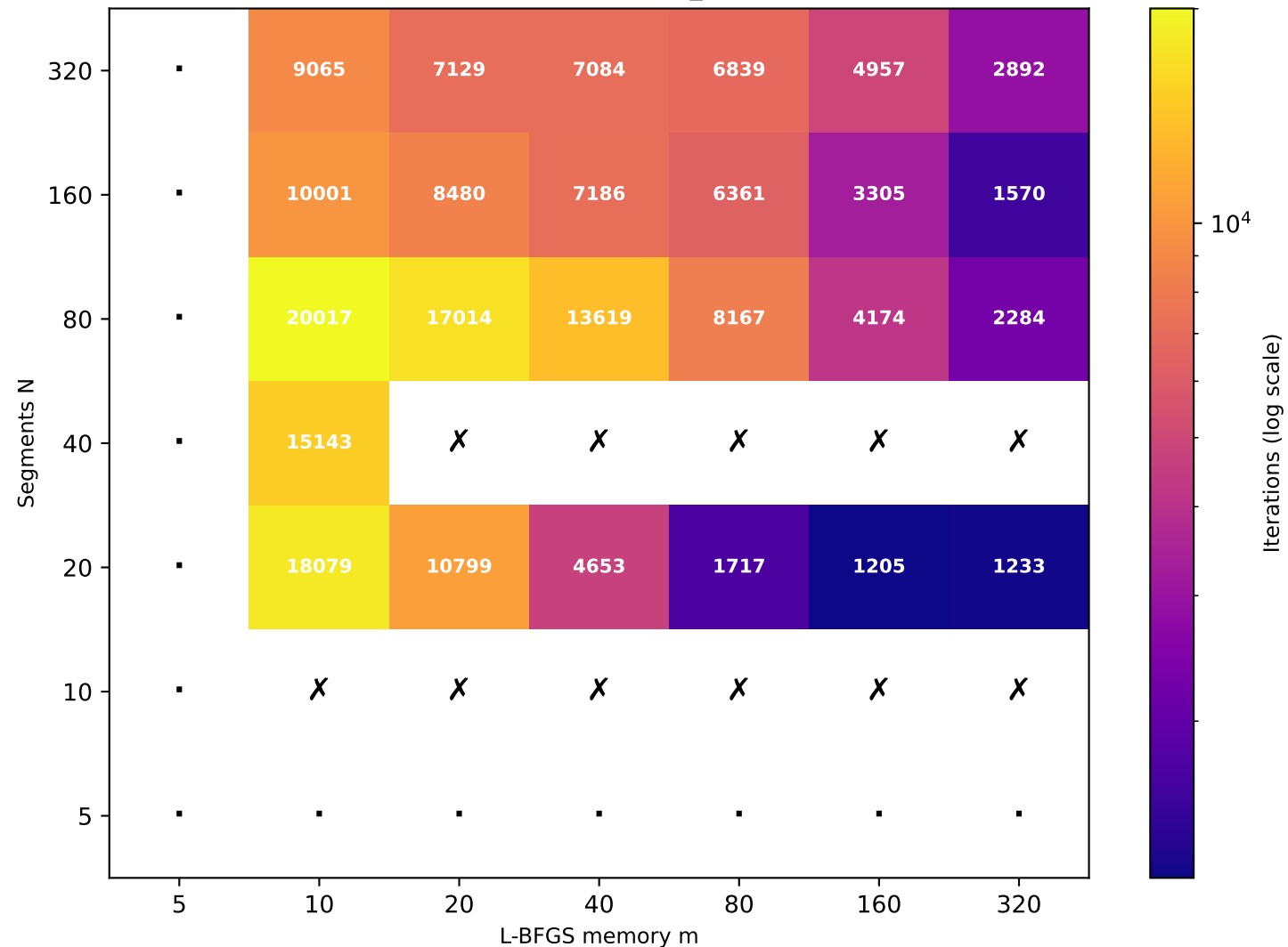
Recurrence T \approx 40.35 (target T=40 , rec_id=33) [25/49 converged]
