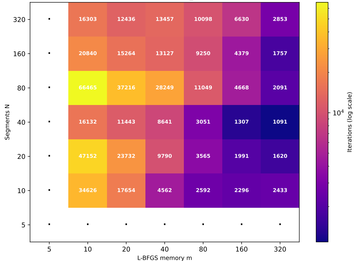
Recurrence T \approx 40.50 (target T=40 , rec_id=34) [36/49 converged]
