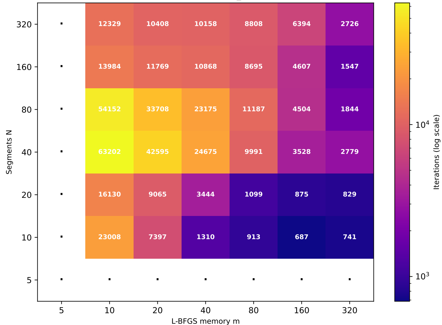
Recurrence T \approx 40.48 (target T=40 , rec_id=35) [36/49 converged]
