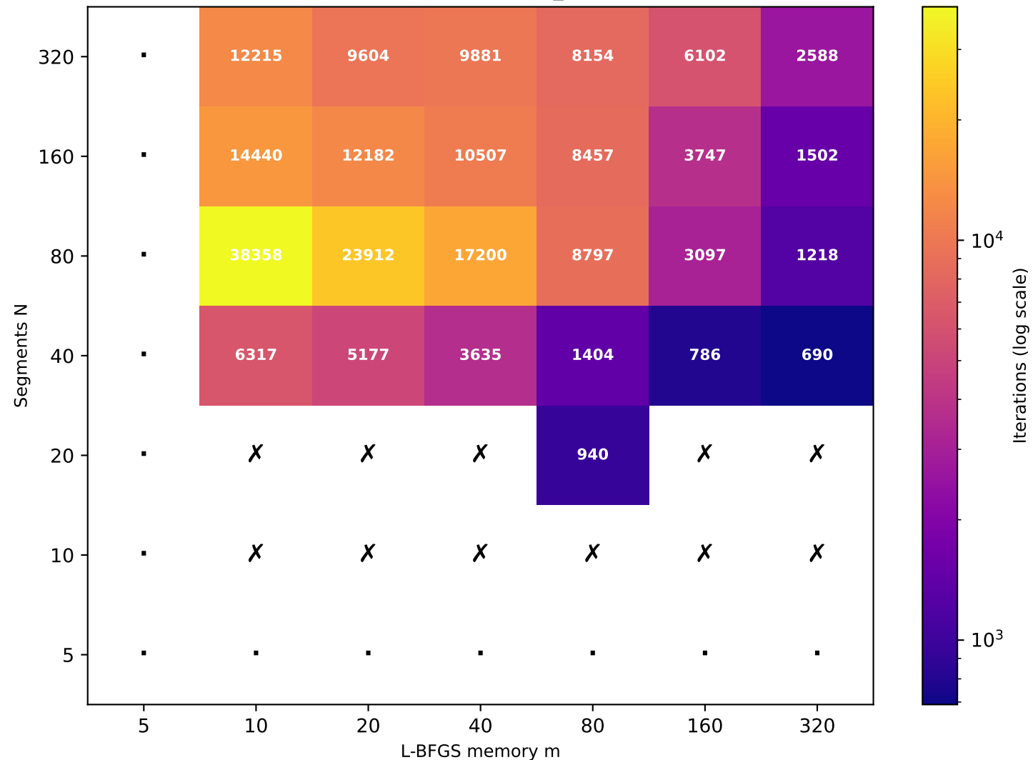
Recurrence T \approx 39.48 (target T=40 , rec_id=36) [25/49 converged]
