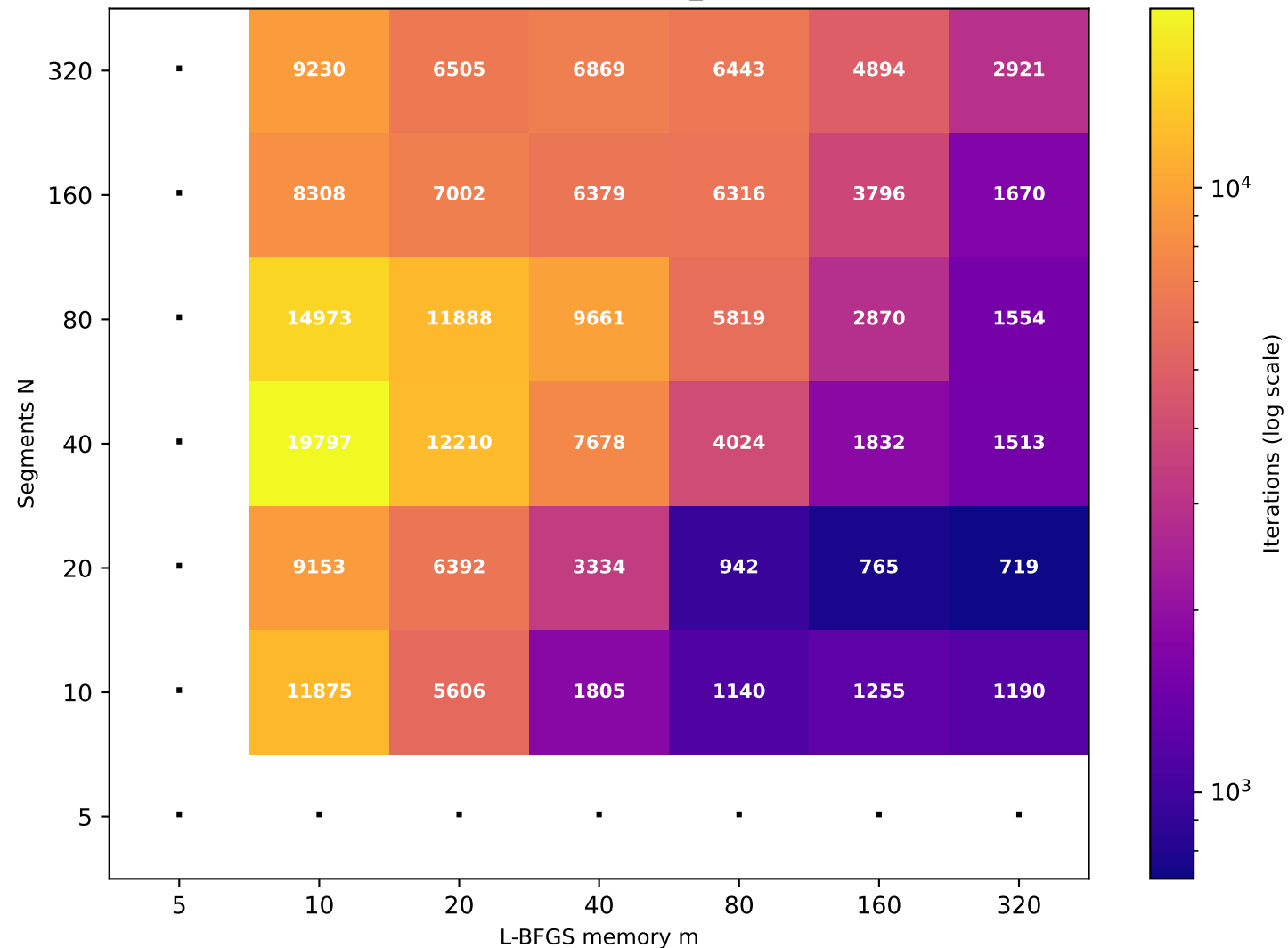
Recurrence T \approx 38.18 (target T=40 , rec_id=39) [36/49 converged]
