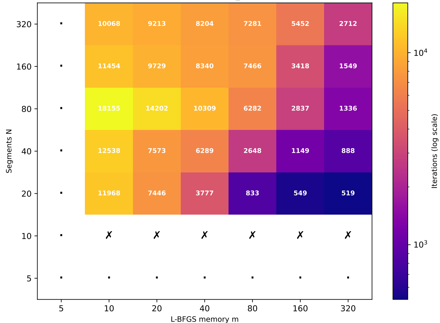
Recurrence T \approx 40.36 (target T=40 , rec_id=40) [30/49 converged]
