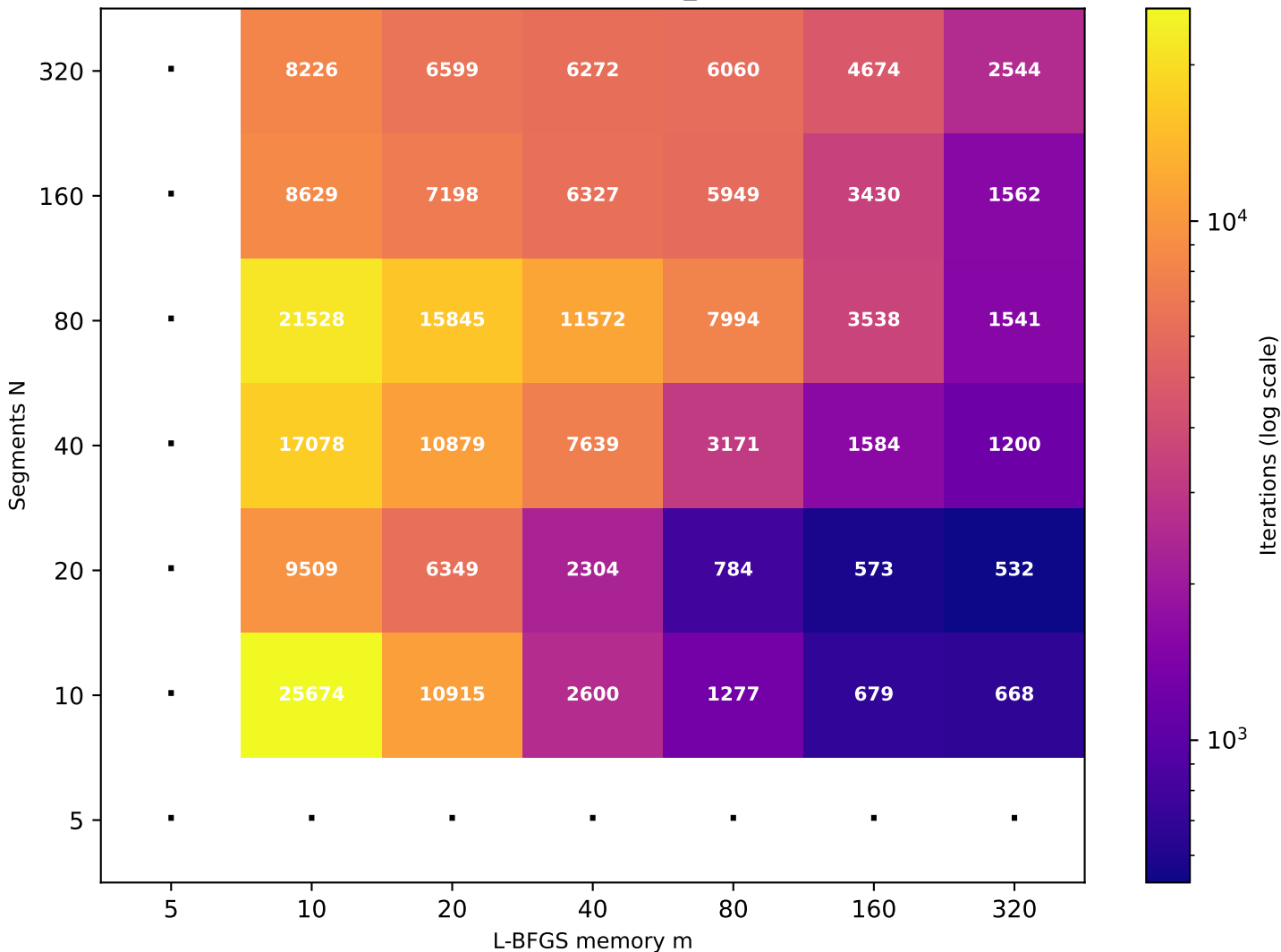
Recurrence T \approx 38.17 (target T=40 , rec_id=41) [36/49 converged]
