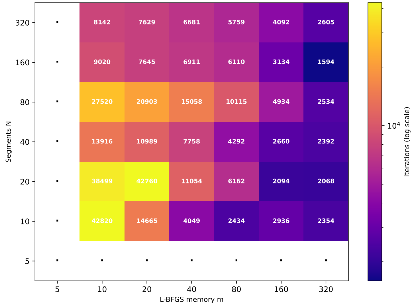
Recurrence T \approx 39.62 (target T=40 , rec_id=43) [36/49 converged]
