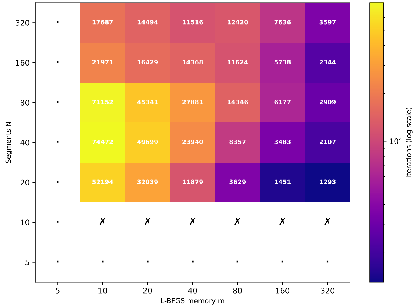
Recurrence T \approx 42.15 (target T=40 , rec_id=44) [30/49 converged]
