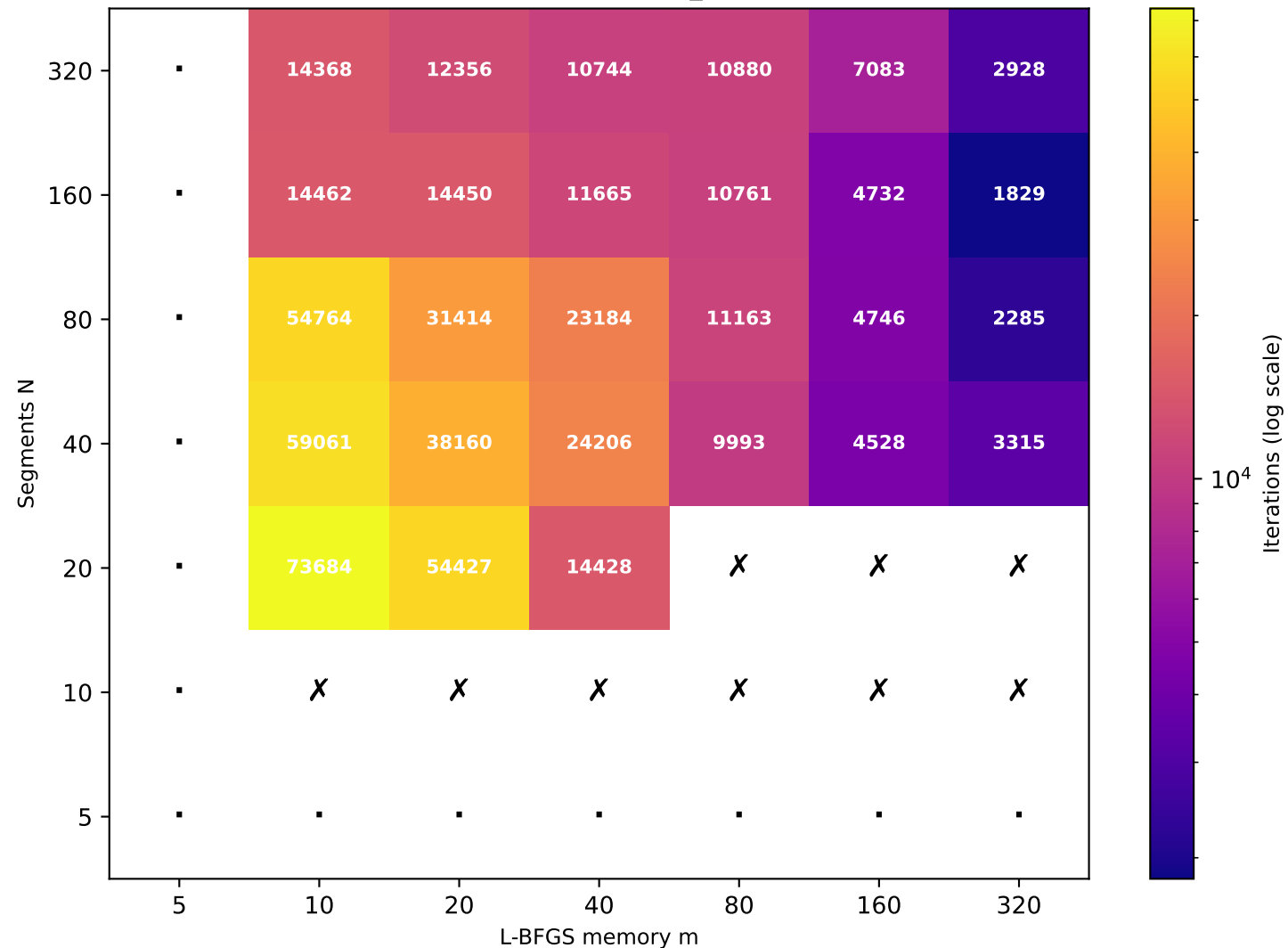
Recurrence T \approx 39.50 (target T=40 , rec_id=49) [27/49 converged]
