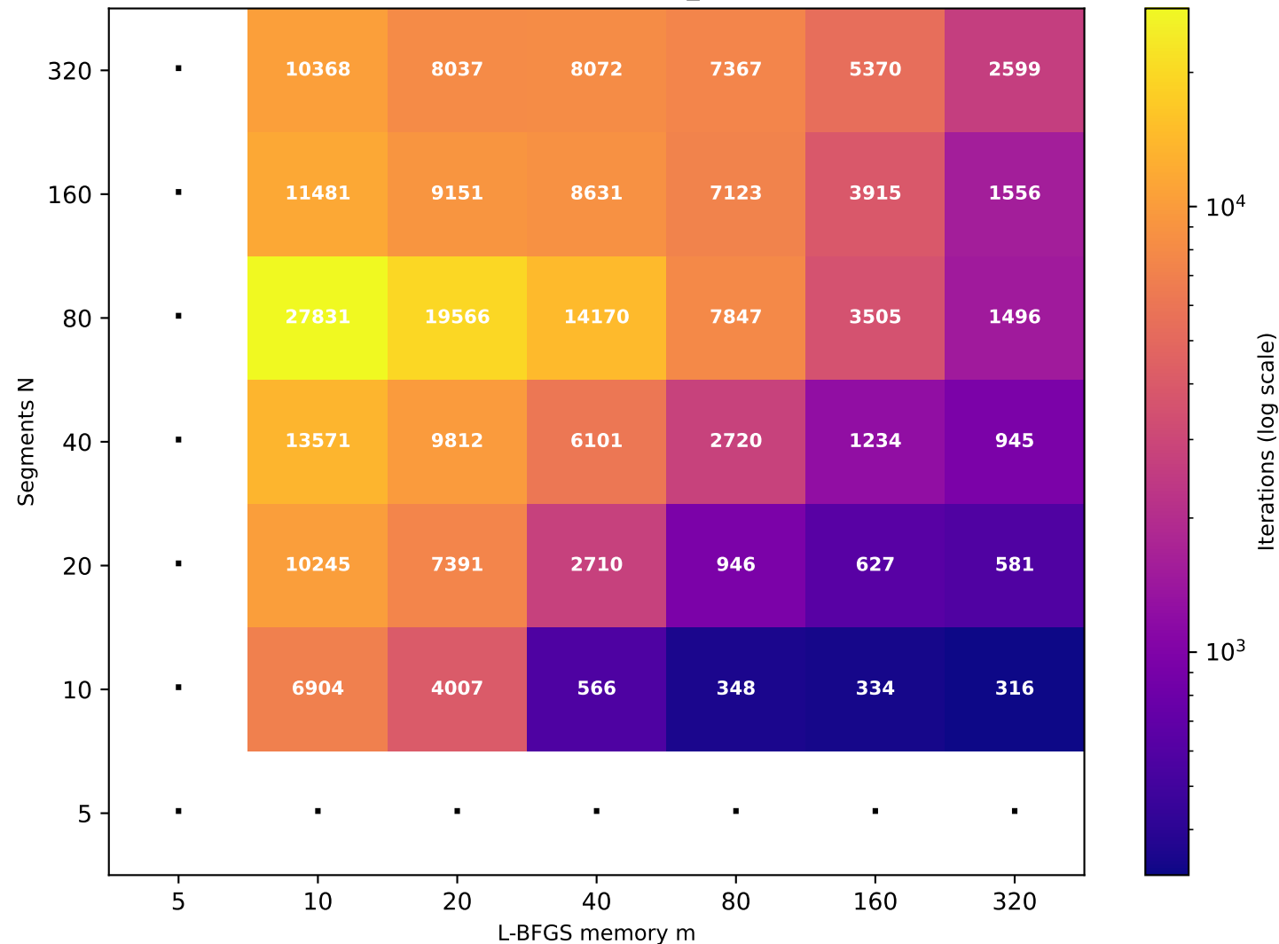
Recurrence T \approx 38.64 (target T=40 , rec_id=54) [36/49 converged]
