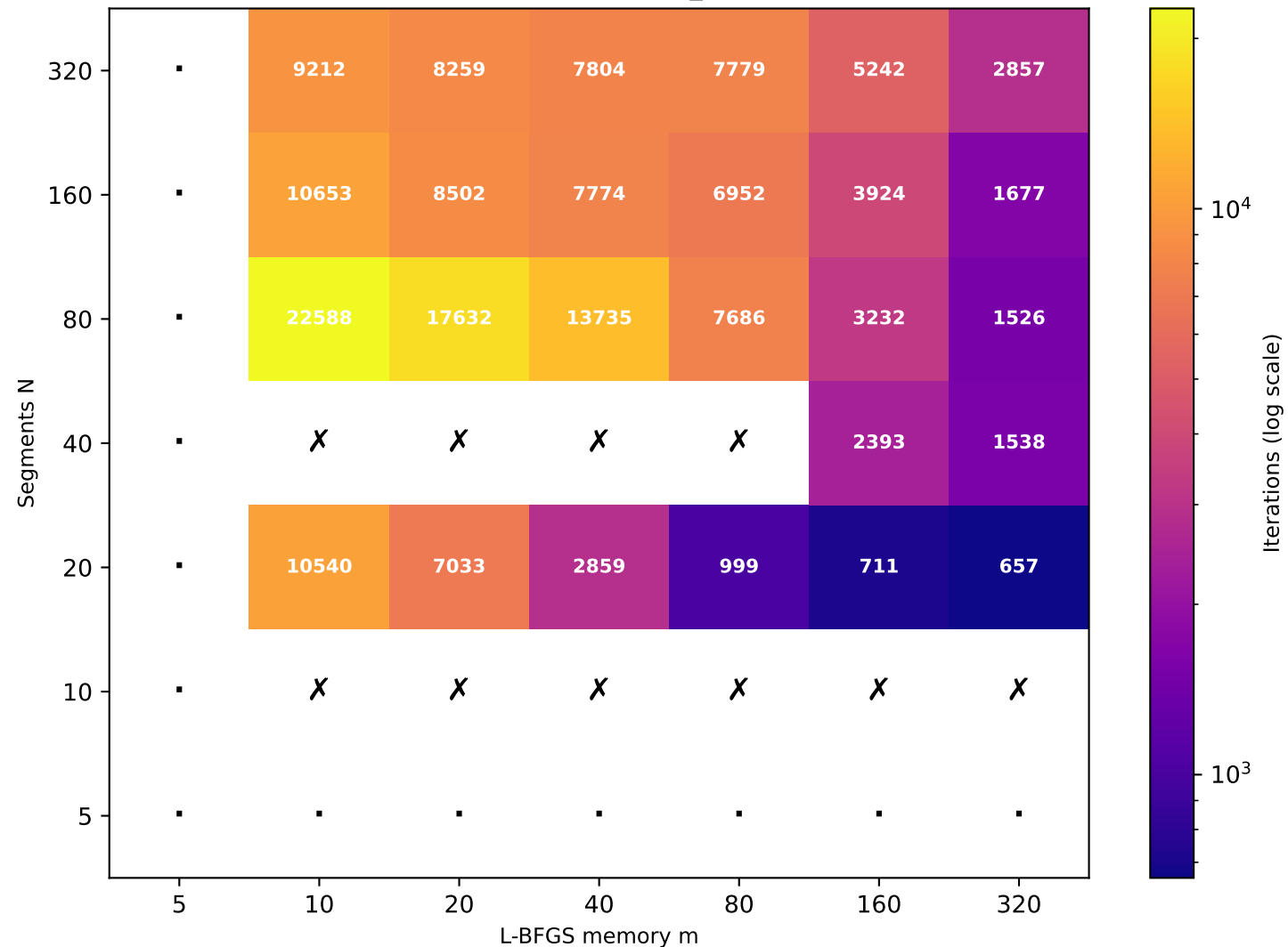
Recurrence T \approx 40.31 (target T=40 , rec_id=56) [26/49 converged]
