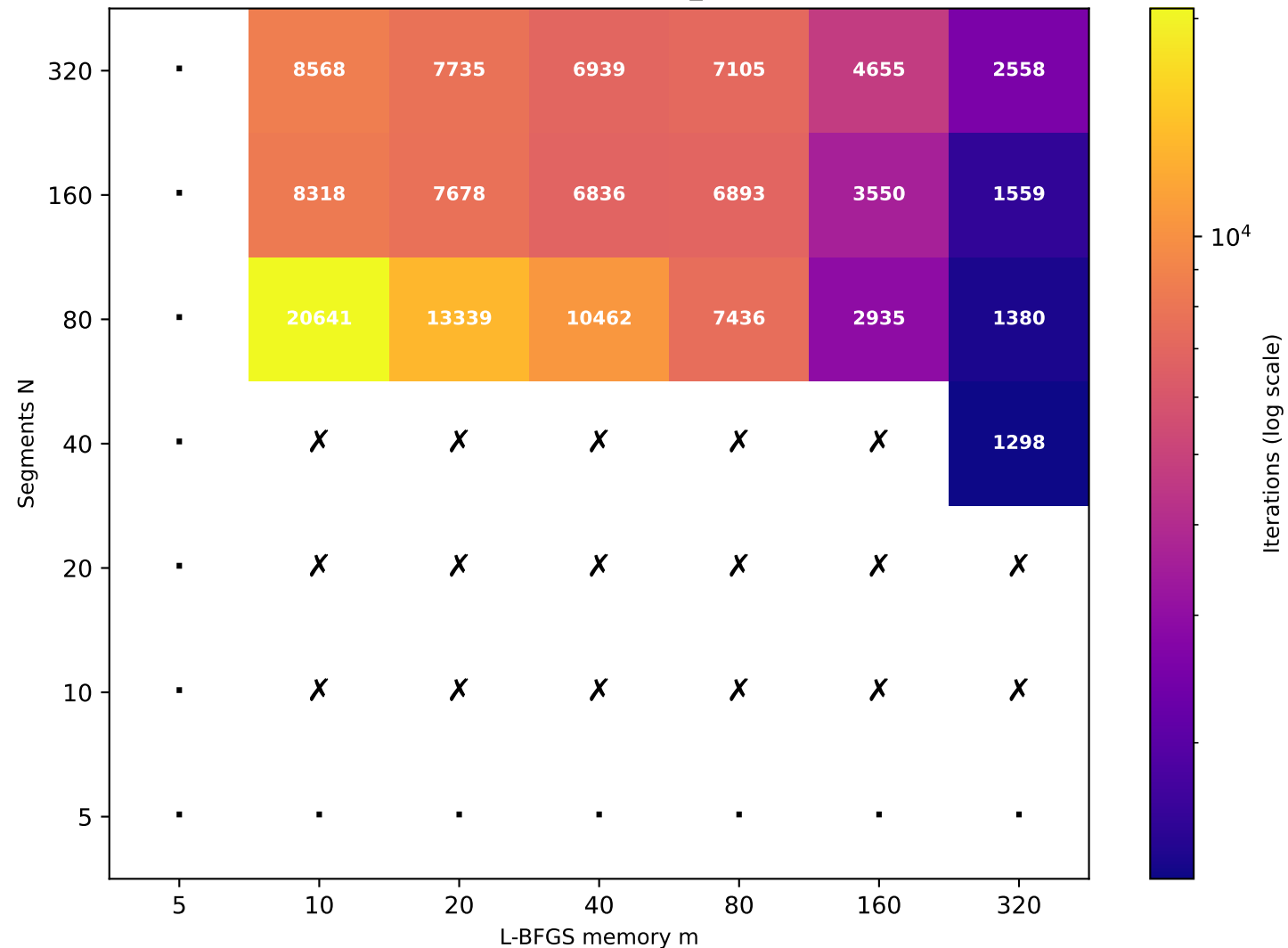
Recurrence T \approx 40.47 (target T=40 , rec_id=59) [19/49 converged]
