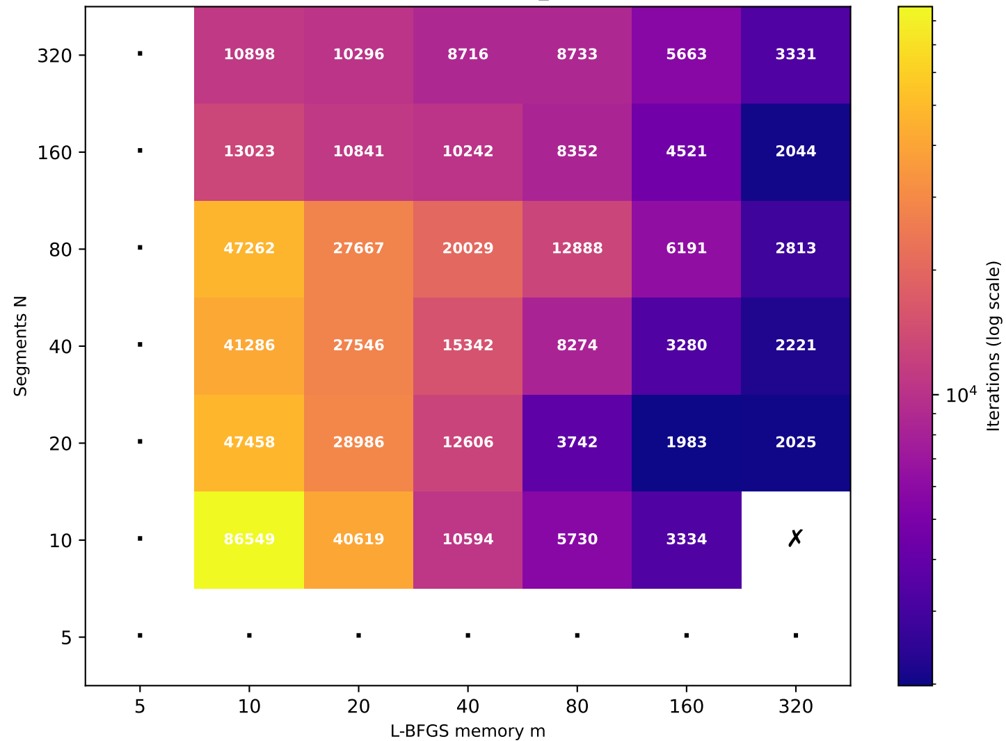
Recurrence T \approx 40.30 (target T=40 , rec_id=60) [35/49 converged]
