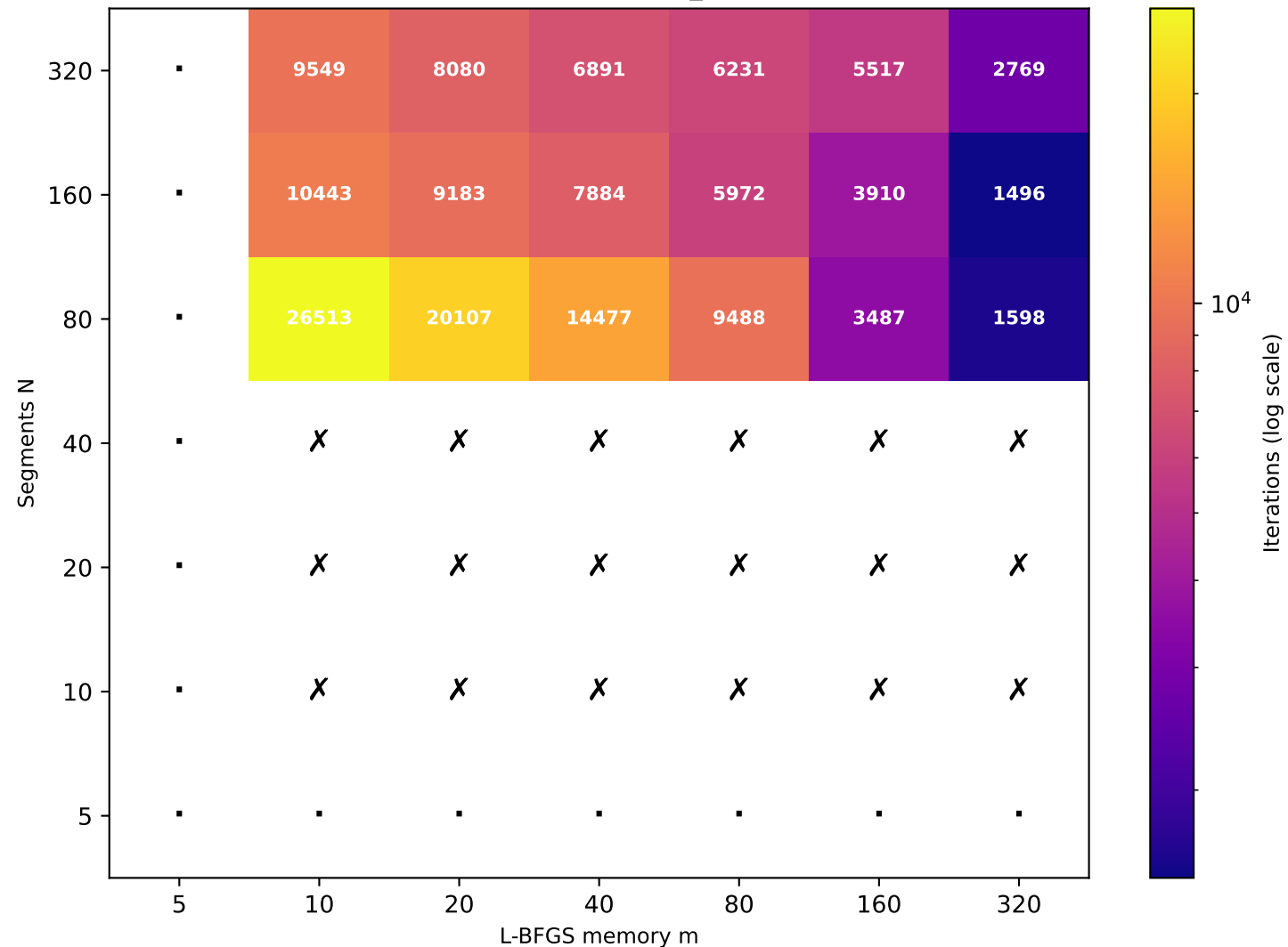
Recurrence T \approx 40.08 (target T=40 , rec_id=61) [18/49 converged]
