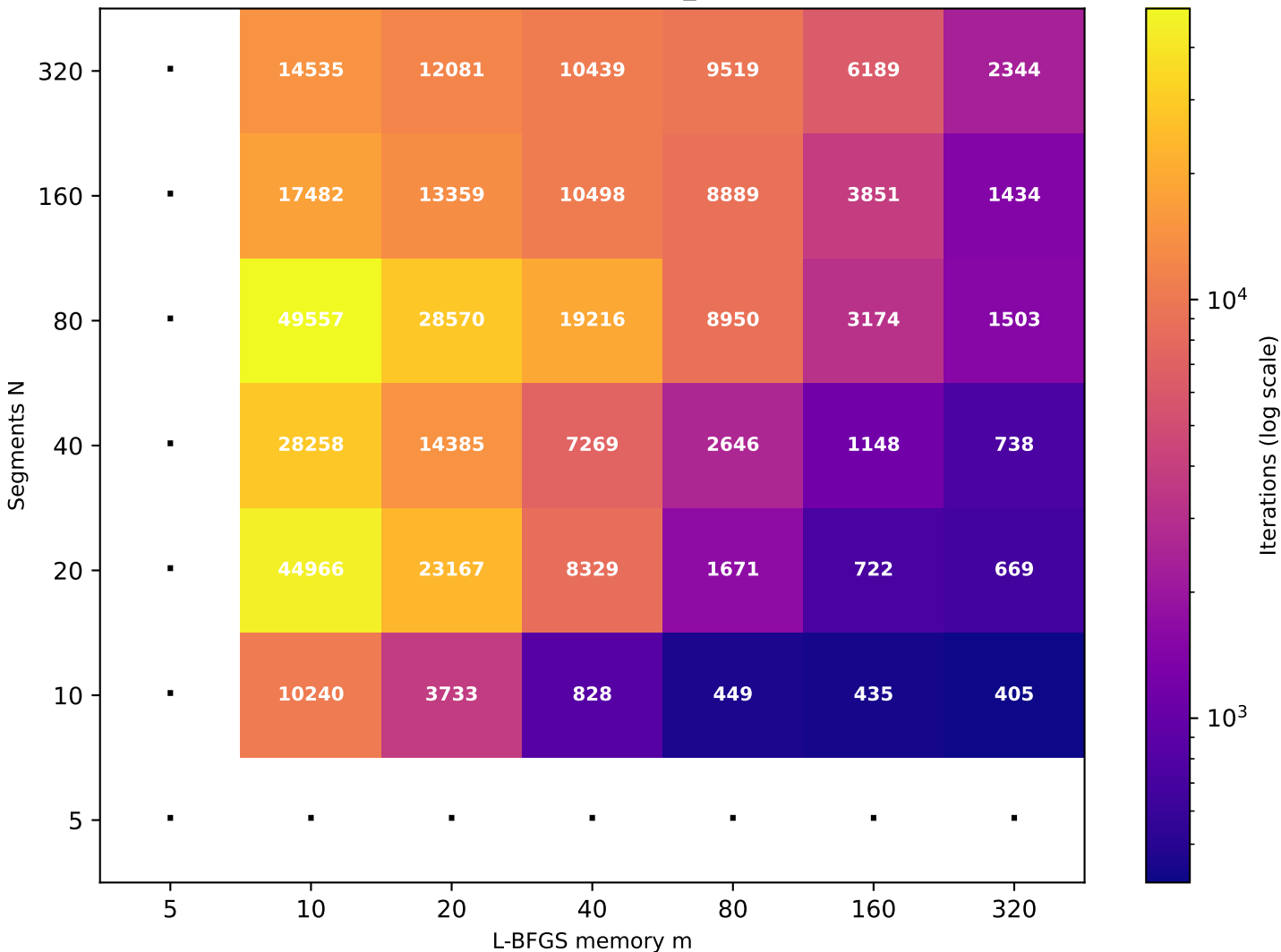
Recurrence T \approx 38.11 (target T=40 , rec_id=64) [36/49 converged]
