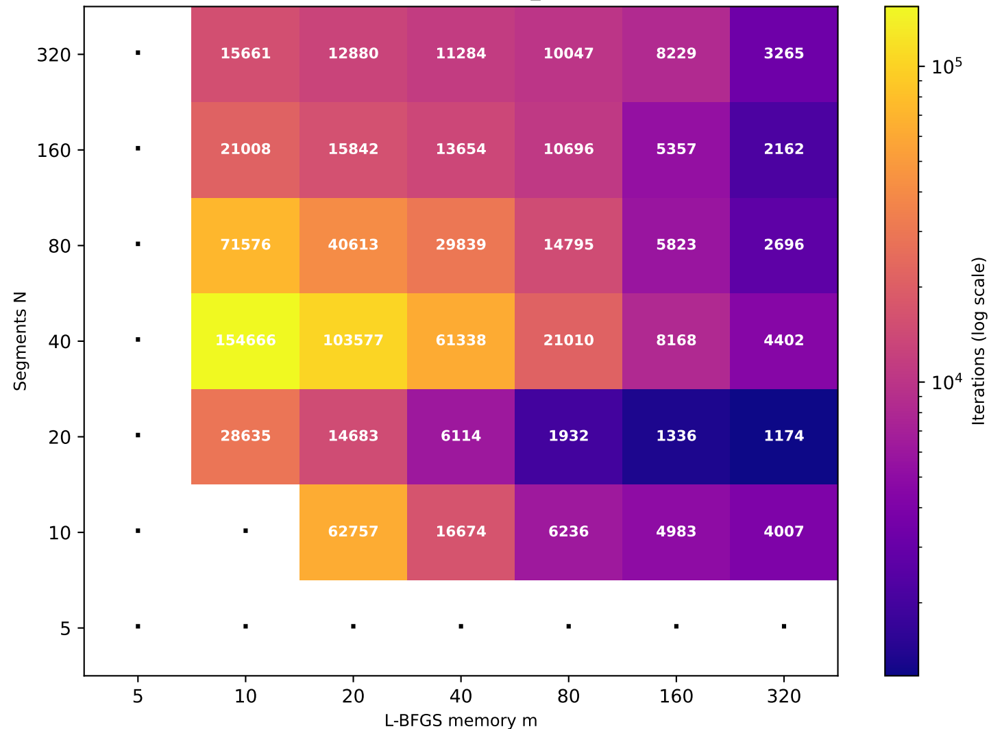
Recurrence T \approx 40.87 (target T=40 , rec_id=65) [35/49 converged]
