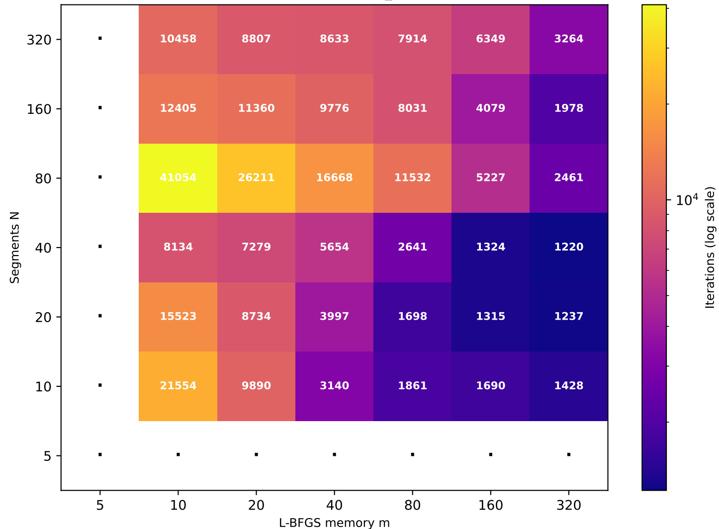
Recurrence T \approx 41.02 (target T=40 , rec_id=68) [36/49 converged]
