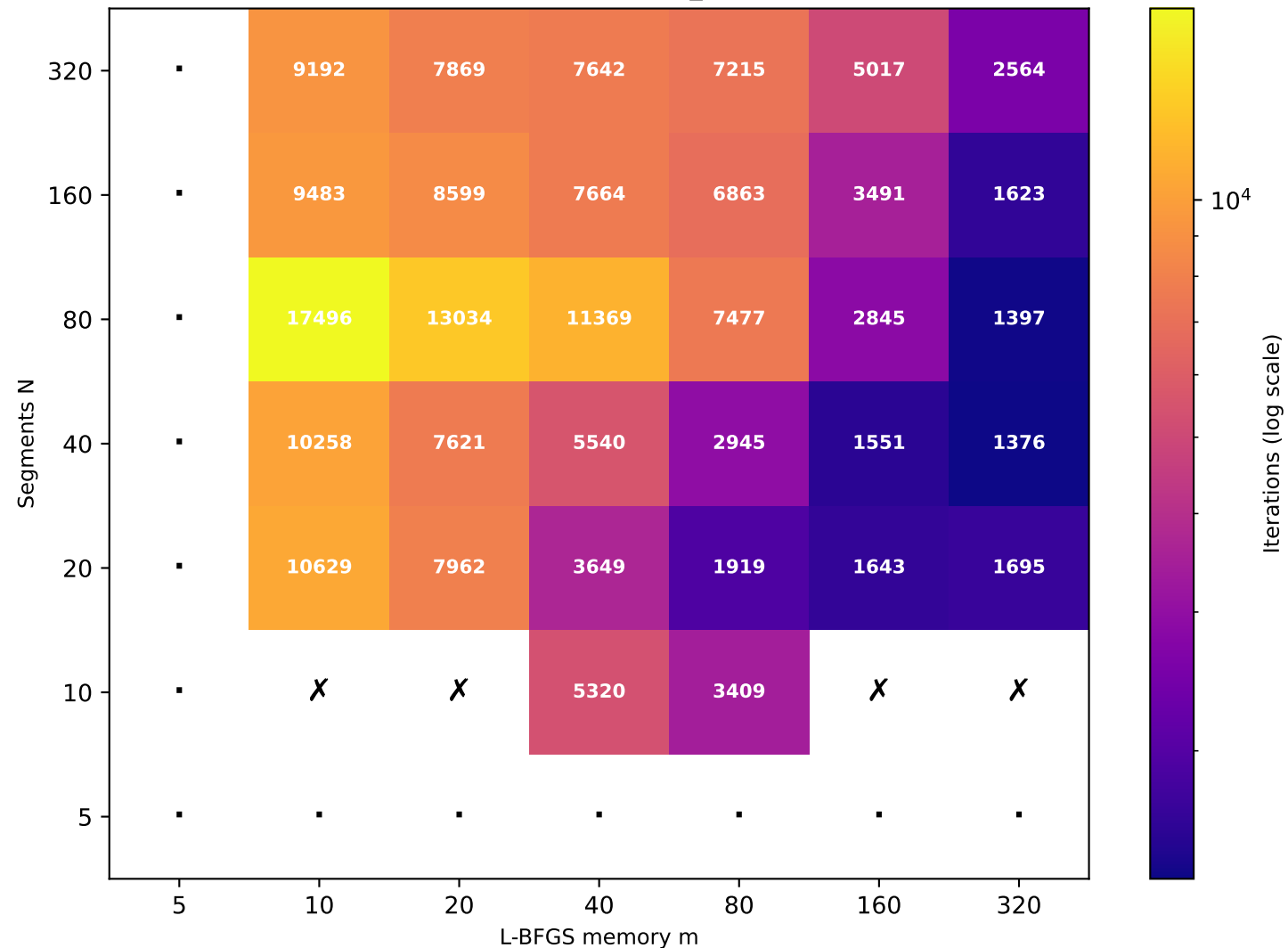
Recurrence T \approx 38.78 (target T=40 , rec_id=69) [32/49 converged]
