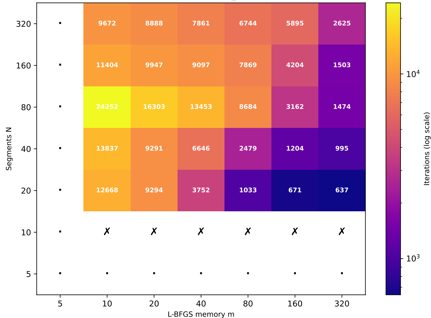
Recurrence T \approx 39.03 (target T=40 , rec_id=70) [30/49 converged]
