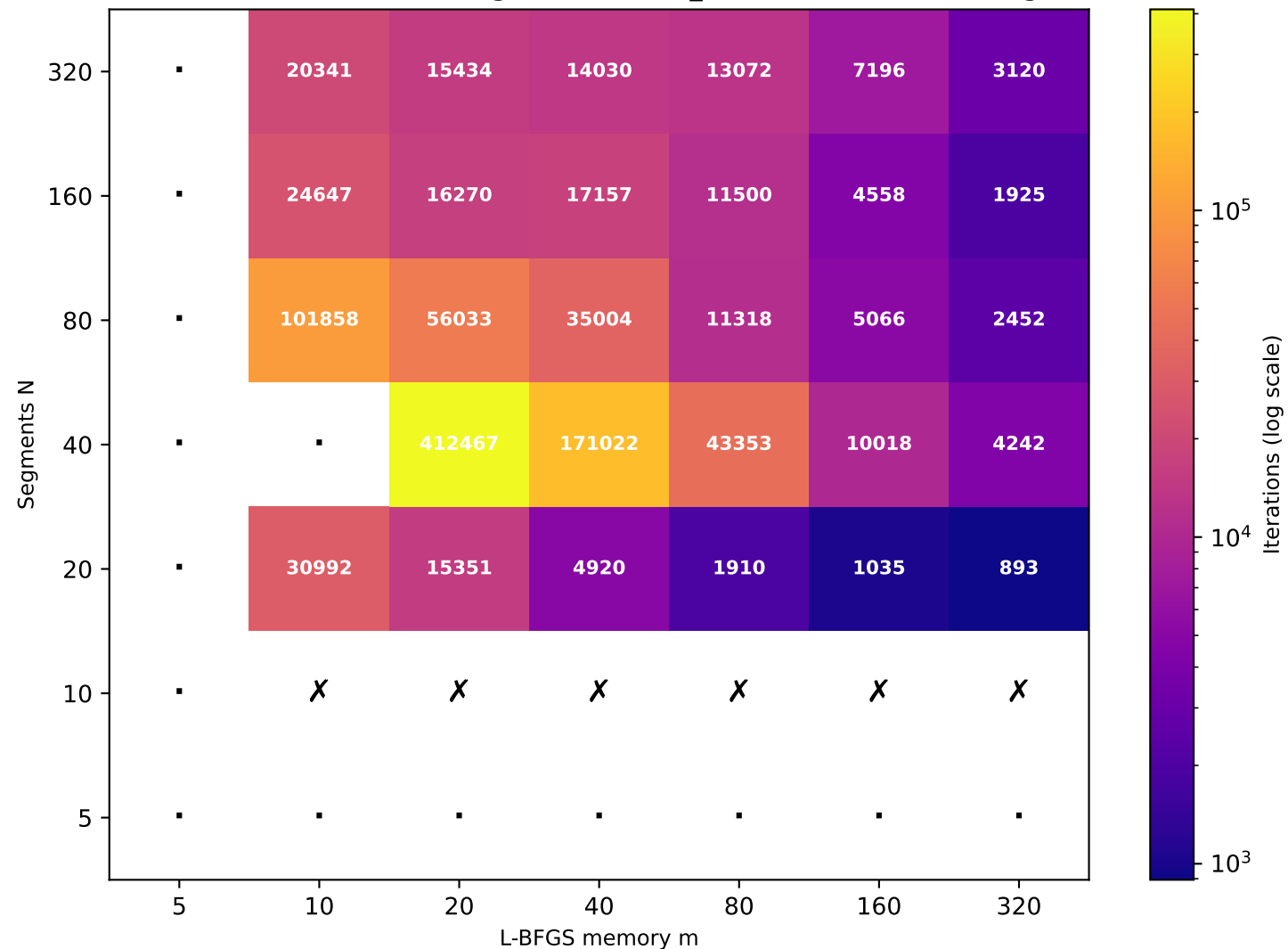
Recurrence T \approx 38.10 (target T=40 , rec_id=76) [29/49 converged]
