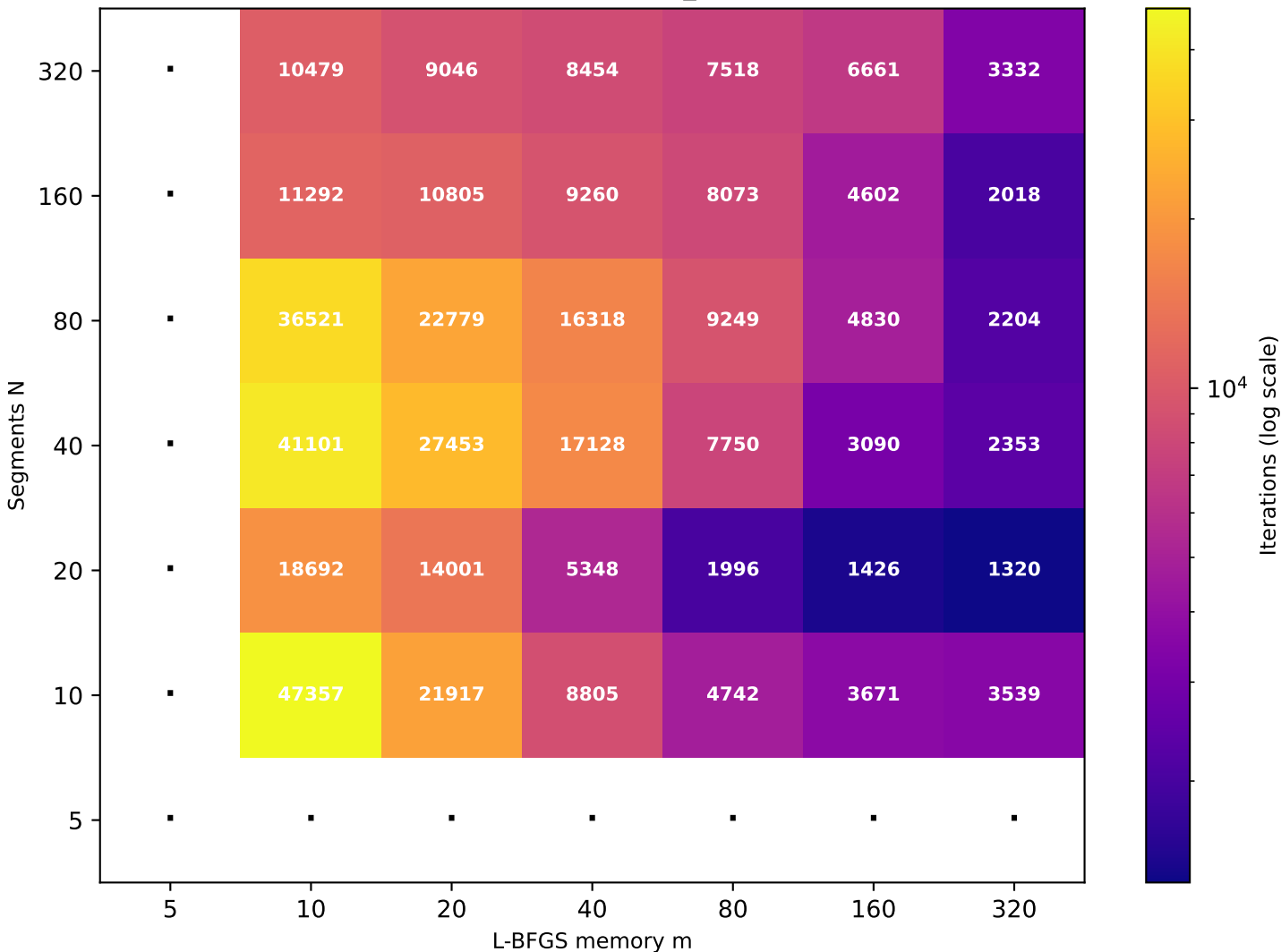
Recurrence T \approx 42.41 (target T=40 , rec_id=79) [36/49 converged]
