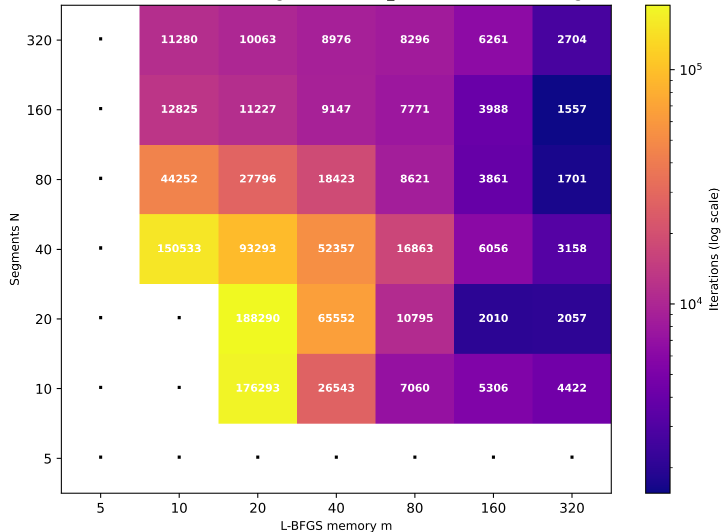
Recurrence T \approx 38.35 (target T=40 , rec_id=82) [34/49 converged]
