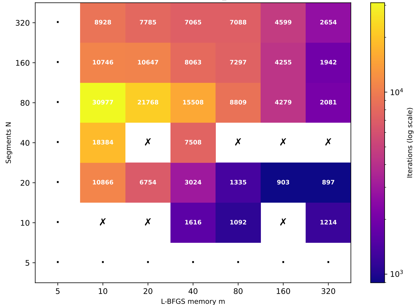
Recurrence T \approx 39.36 (target T=40 , rec_id=83) [29/49 converged]
