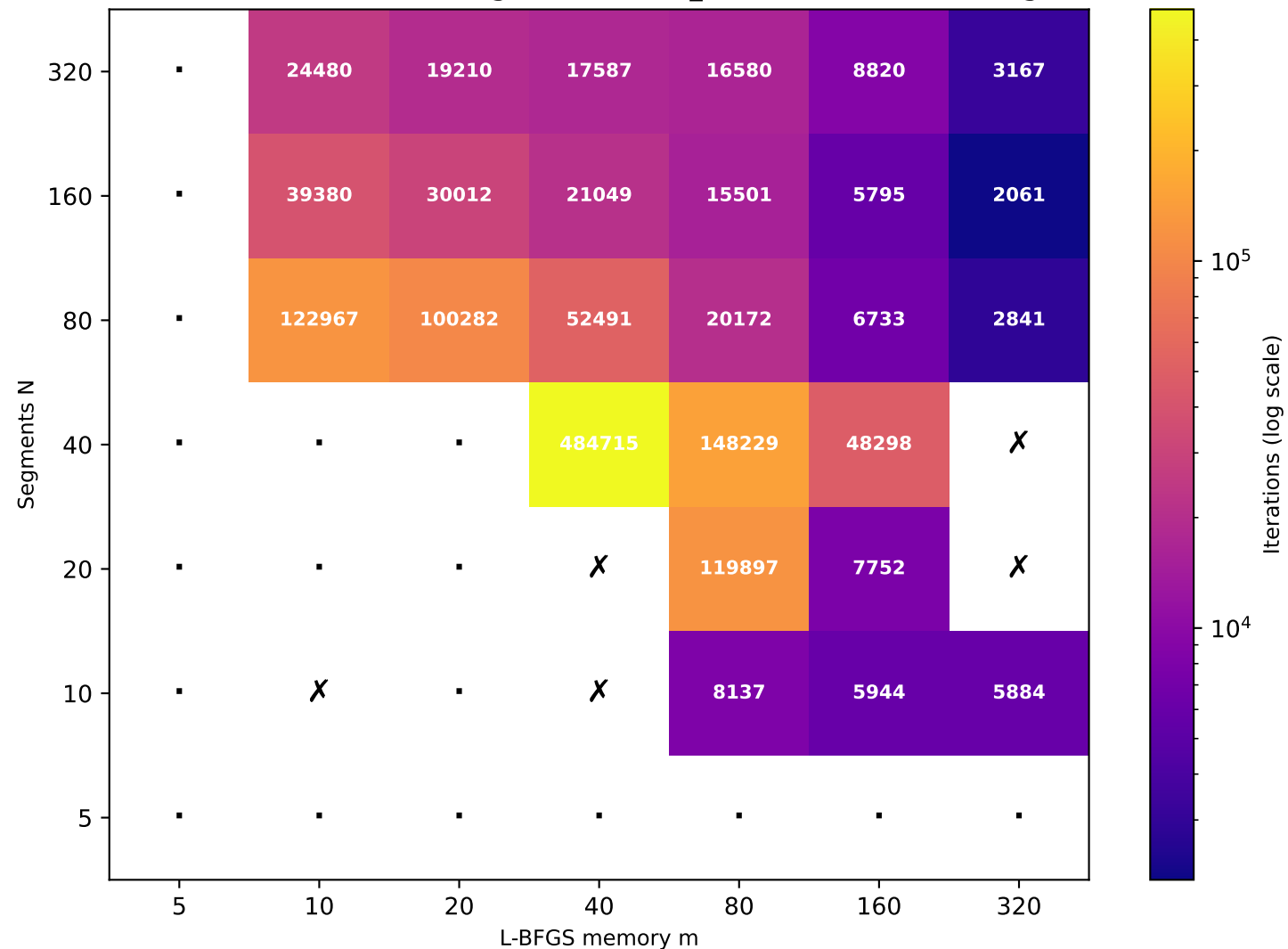
Recurrence T \approx 41.65 (target T=40 , rec_id=88) [26/49 converged]
