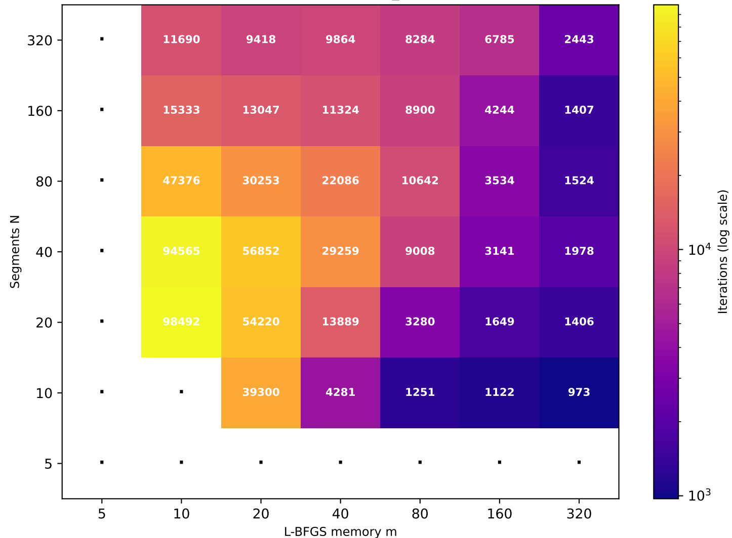
Recurrence T \approx 40.77 (target T=40 , rec_id=95) [35/49 converged]
