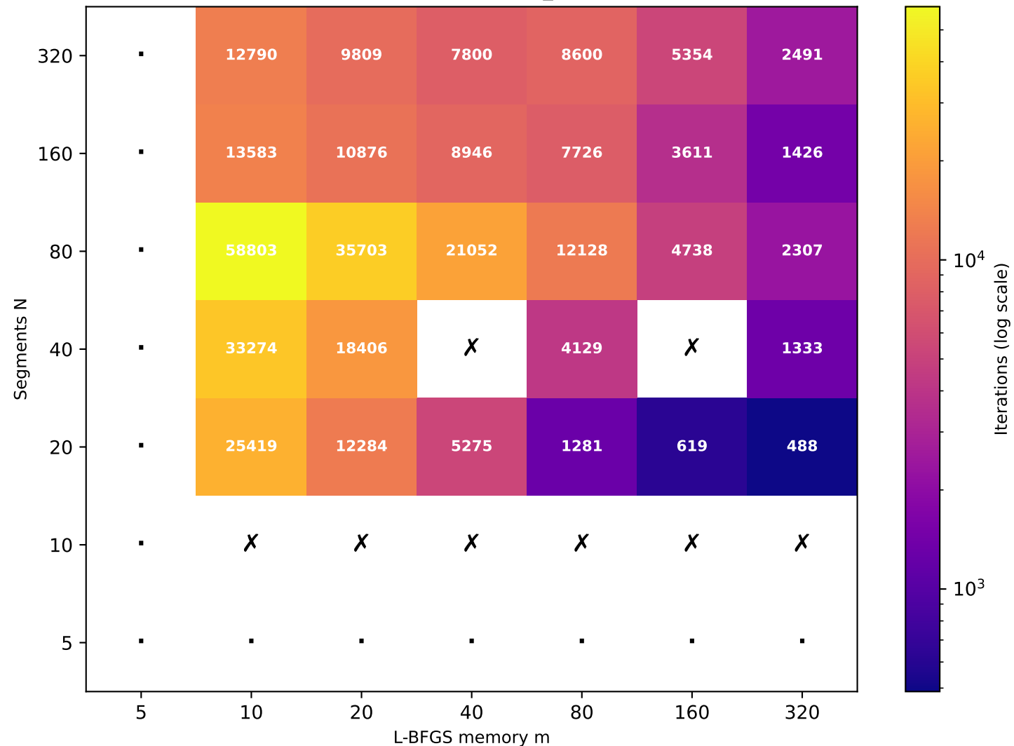
Recurrence T \approx 38.32 (target T=40 , rec_id=96) [28/49 converged]
