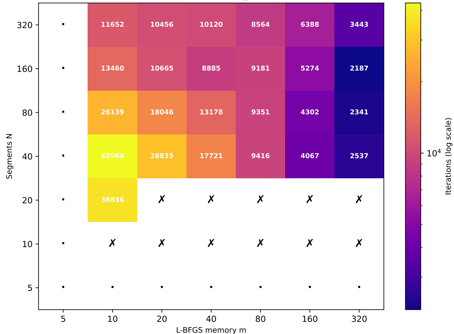
Recurrence T \approx 40.91 (target T=40 , rec_id=98) [25/49 converged]
