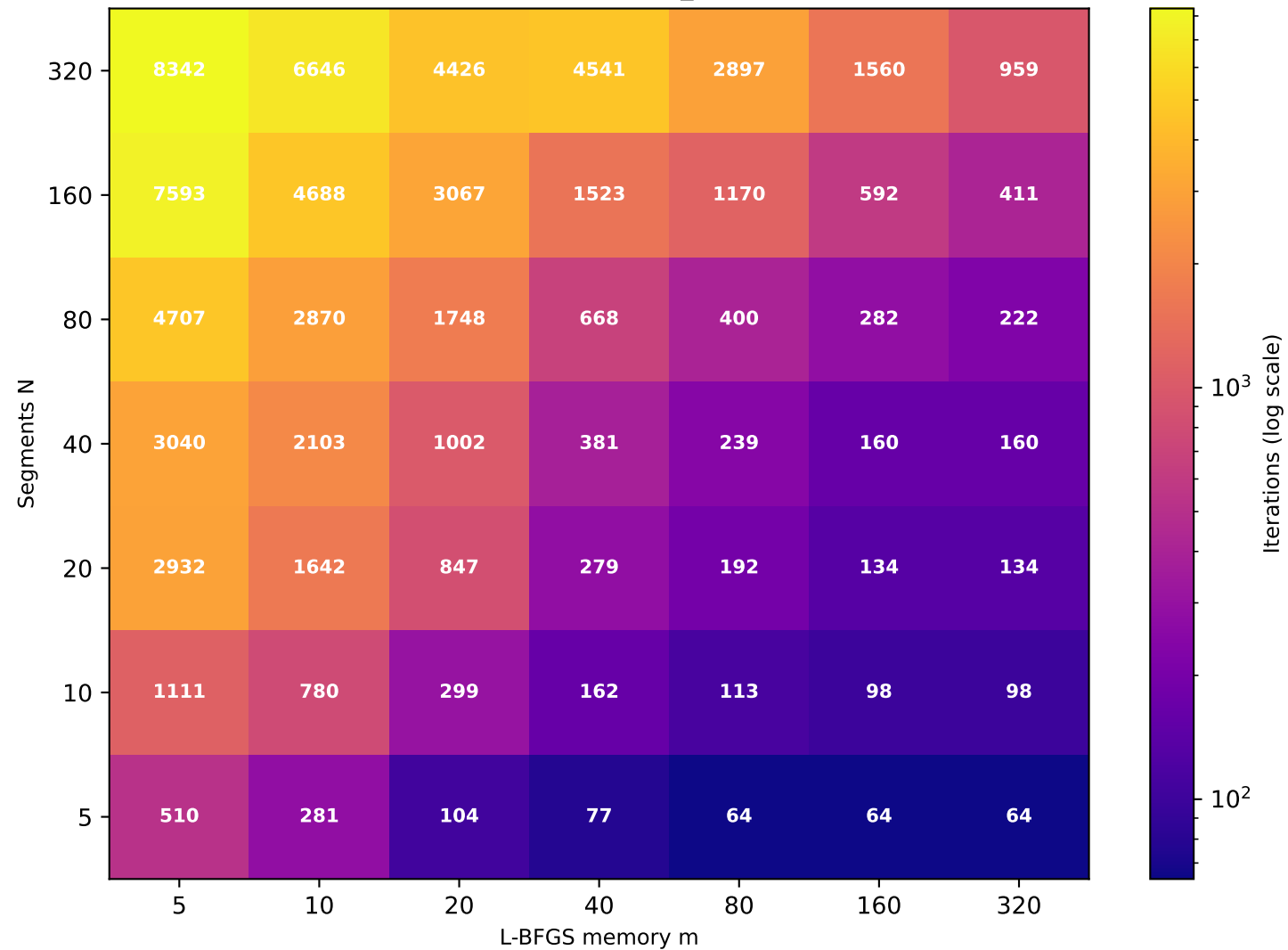
Recurrence T \approx 5.37 (target T=5 , rec_id=2) [49/49 converged]
