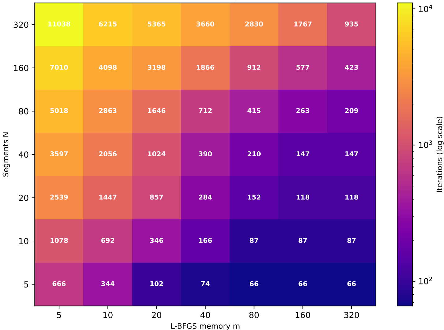
Recurrence T \approx 5.37 (target T=5 , rec_id=3) [49/49 converged]
