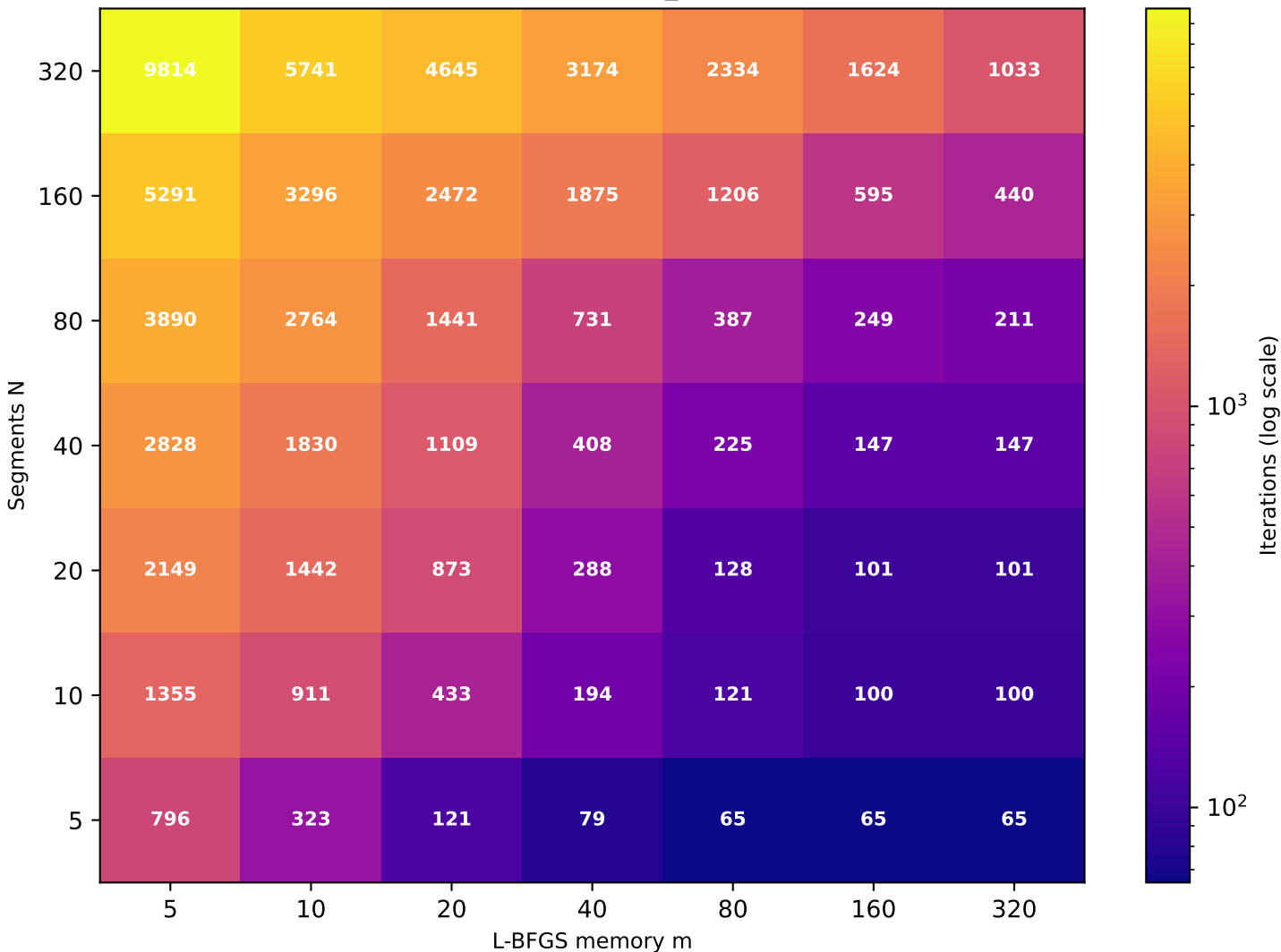
Recurrence T \approx 5.43 (target T=5 , rec_id=10) [49/49 converged]
