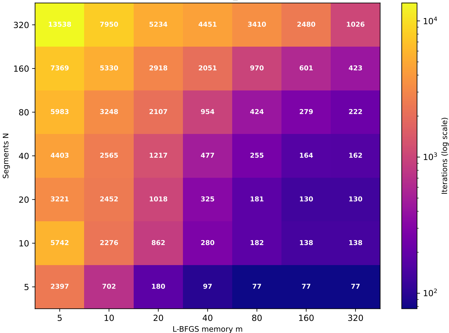
Recurrence T \approx 5.37 (target T=5 , rec_id=11) [49/49 converged]
