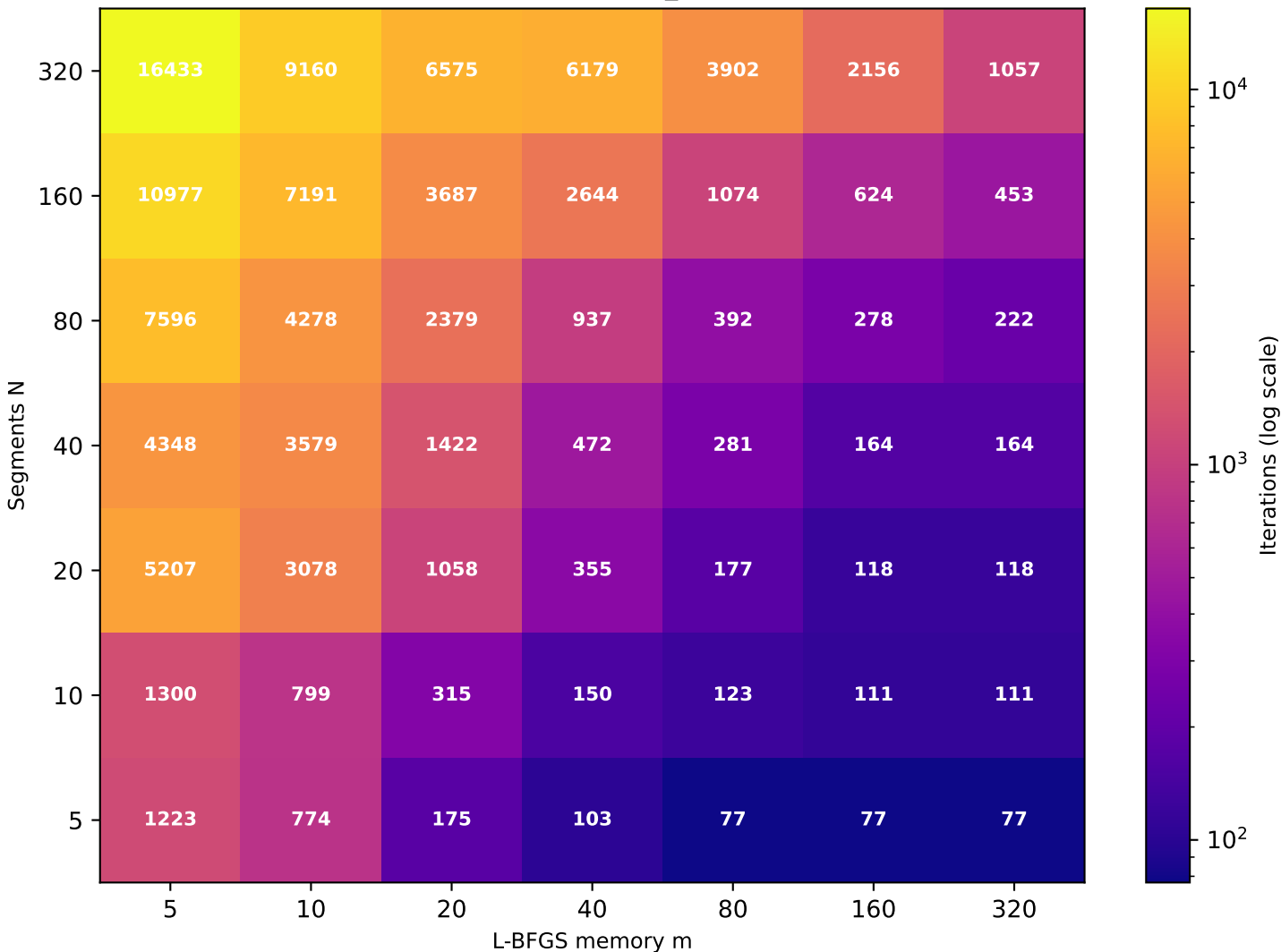
Recurrence T \approx 5.99 (target T=5 , rec_id=13) [49/49 converged]
