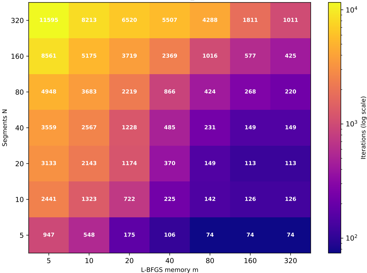
Recurrence T \approx 5.33 (target T=5 , rec_id=30) [49/49 converged]
