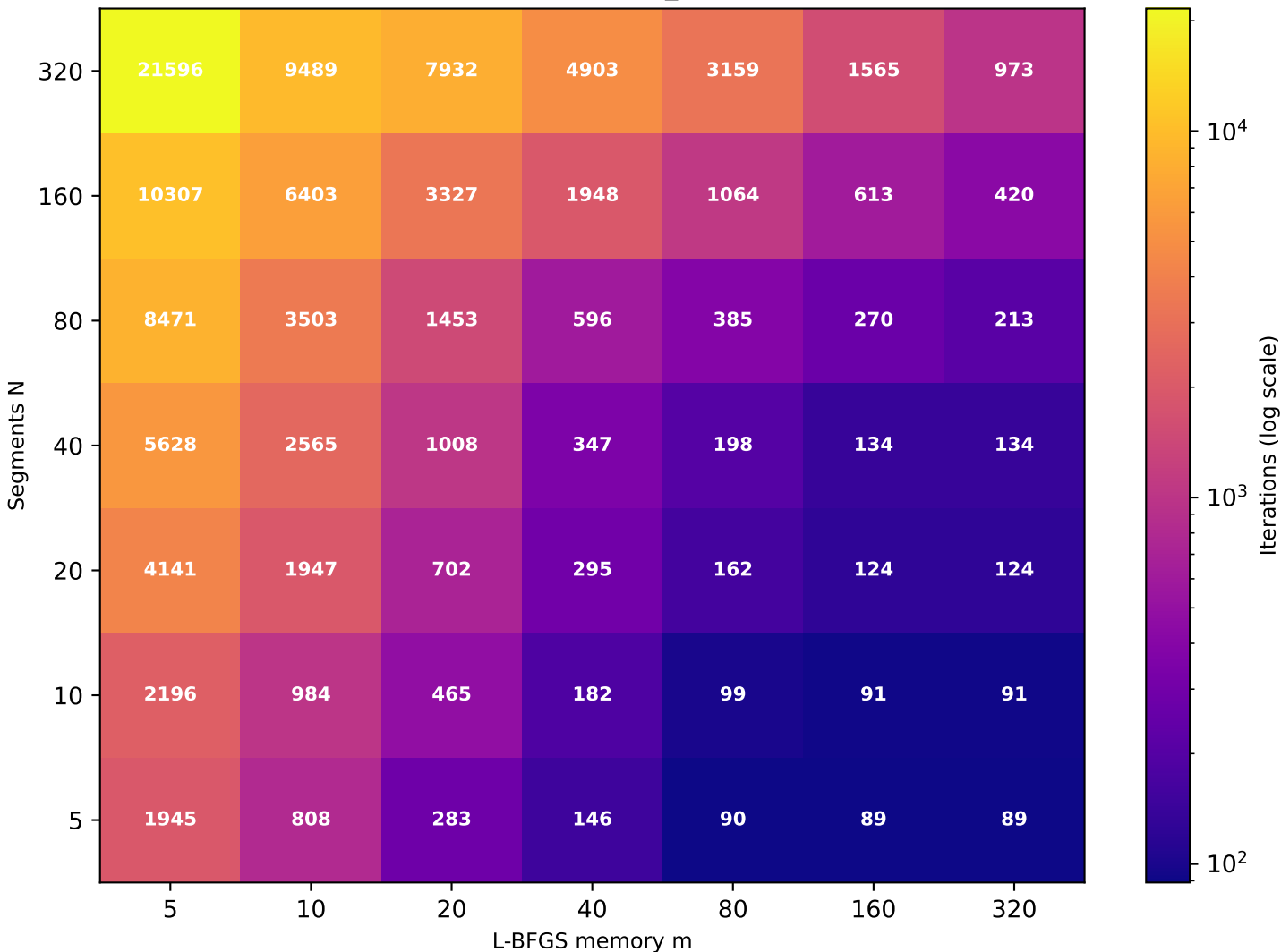
Recurrence T \approx 5.10 (target T=5 , rec_id=31) [49/49 converged]
