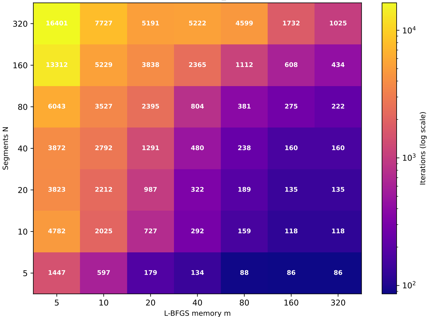
Recurrence T \approx 5.30 (target T=5 , rec_id=33) [49/49 converged]
