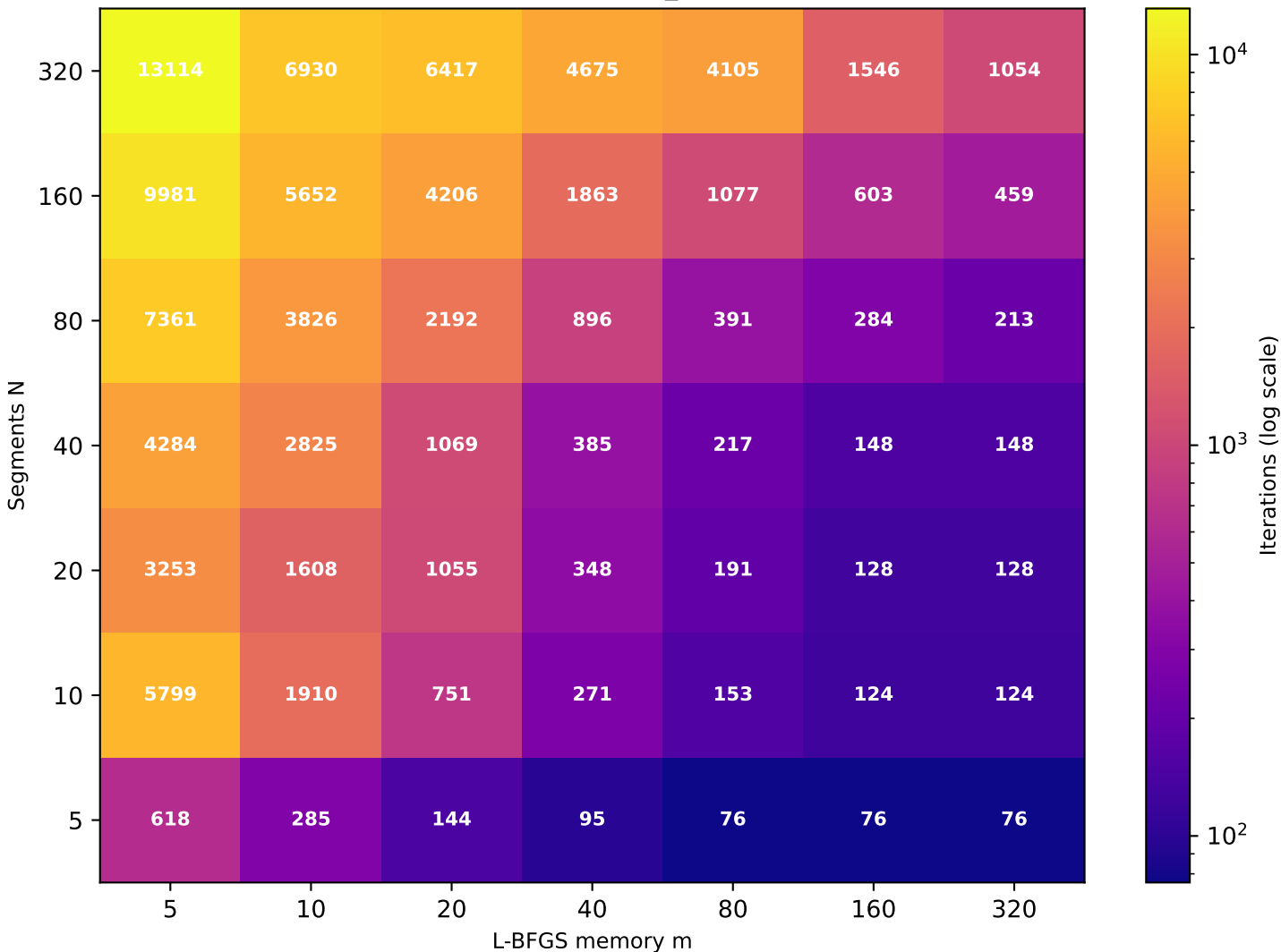
Recurrence T \approx 5.30 (target T=5 , rec_id=41) [49/49 converged]
