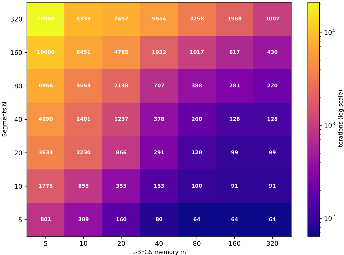
Recurrence T \approx 4.57 (target T=5 , rec_id=43) [49/49 converged]
