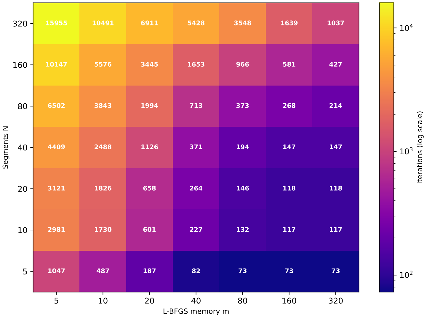
Recurrence T \approx 4.57 (target T=5 , rec_id=45) [49/49 converged]
