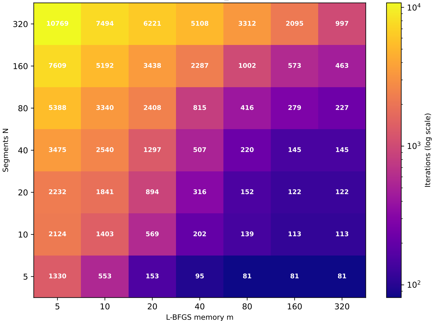
Recurrence T \approx 5.39 (target T=5 , rec_id=48) [49/49 converged]
