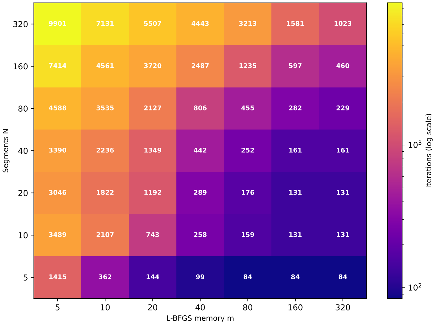
Recurrence T \approx 5.39 (target T=5 , rec_id=50) [49/49 converged]
