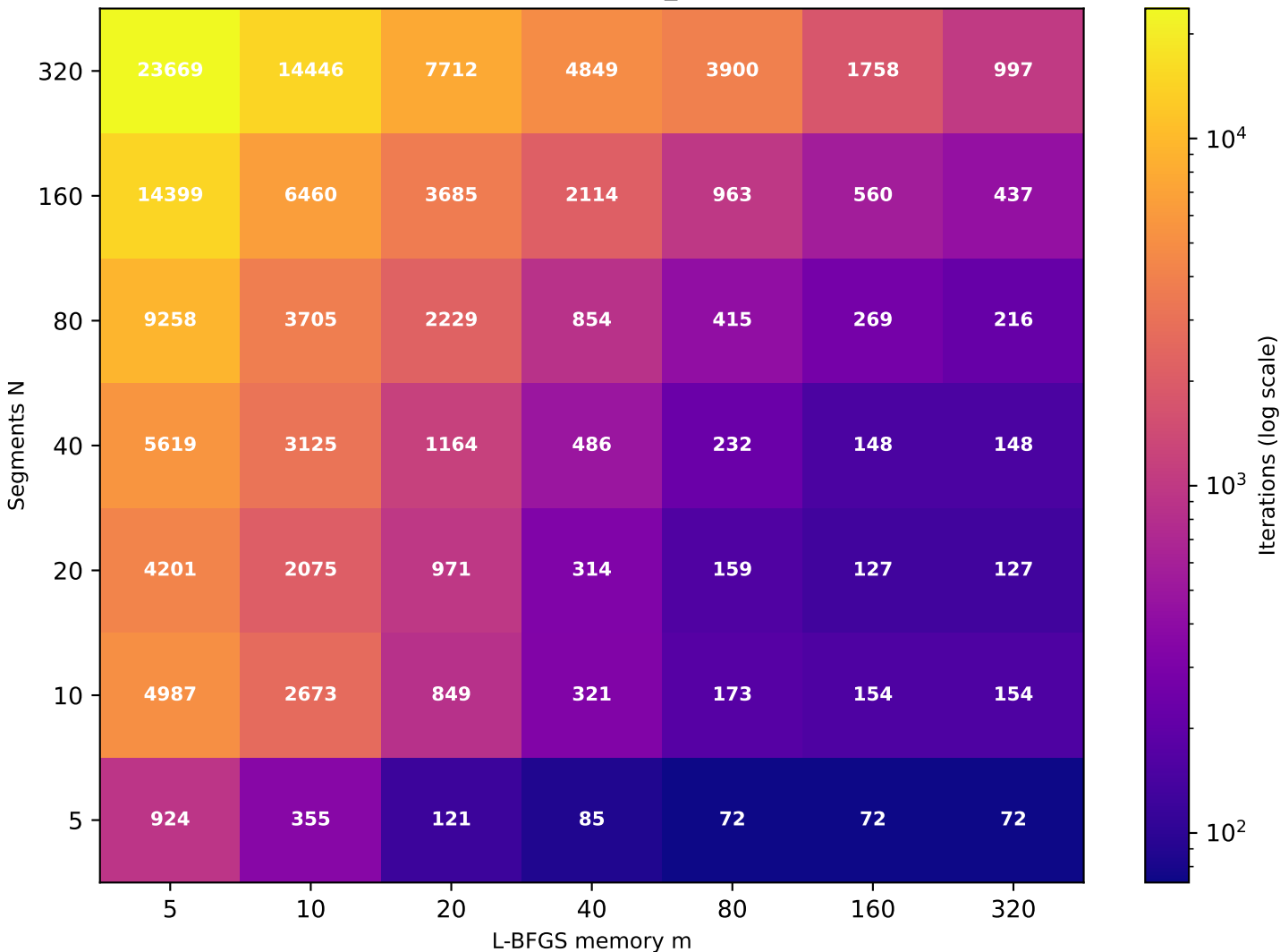
Recurrence T \approx 5.23 (target T=5 , rec_id=51) [49/49 converged]
