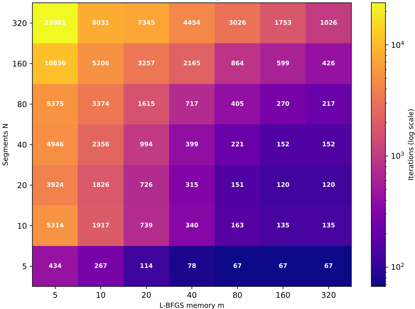
Recurrence T \approx 5.78 (target T=5 , rec_id=54) [49/49 converged]
