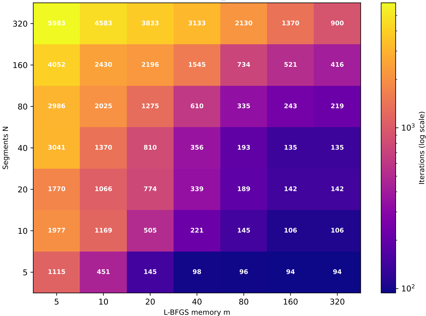
Recurrence T \approx 4.68 (target T=5 , rec_id=55) [49/49 converged]
