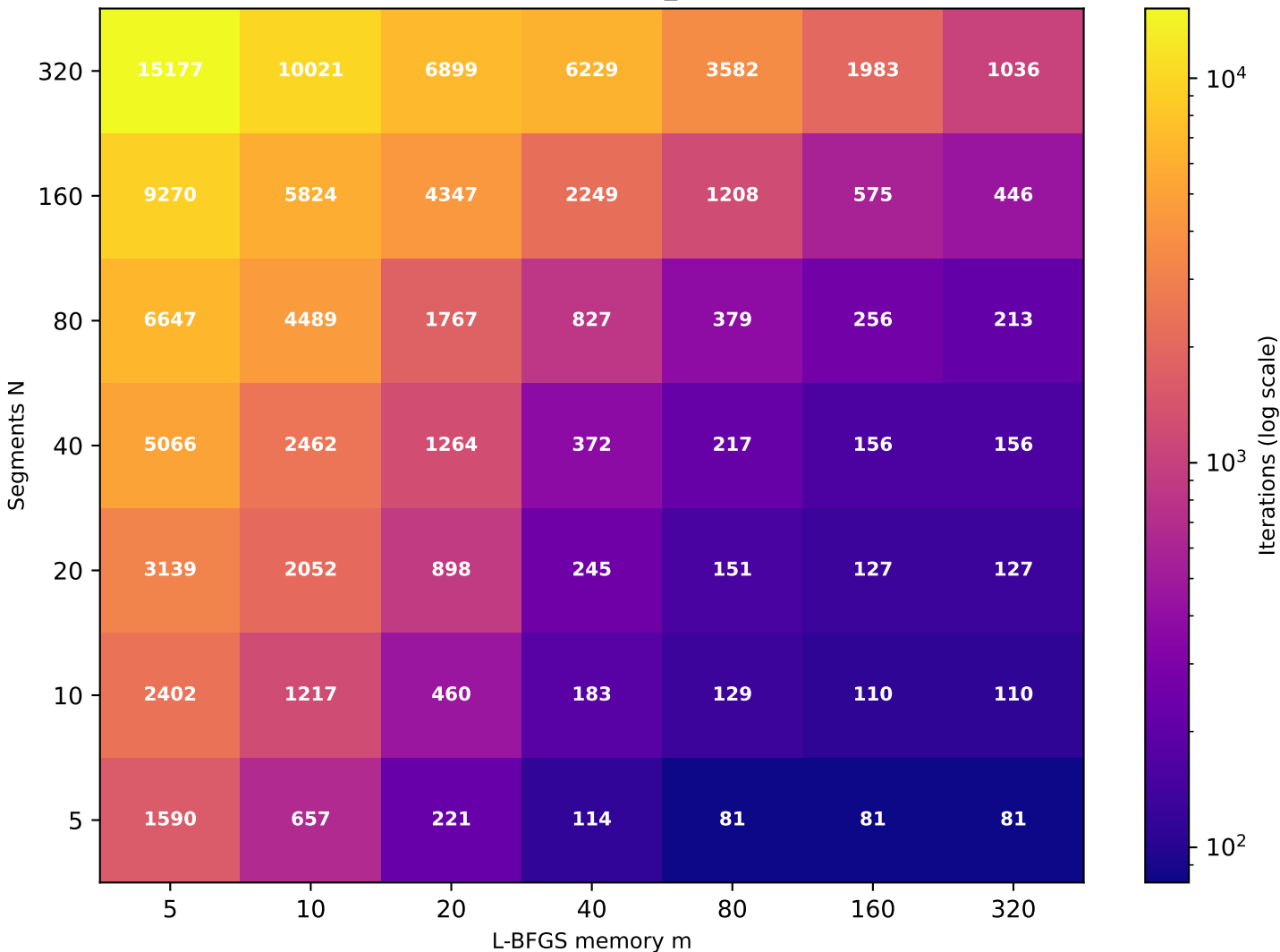
Recurrence T \approx 4.59 (target T=5 , rec_id=56) [49/49 converged]
