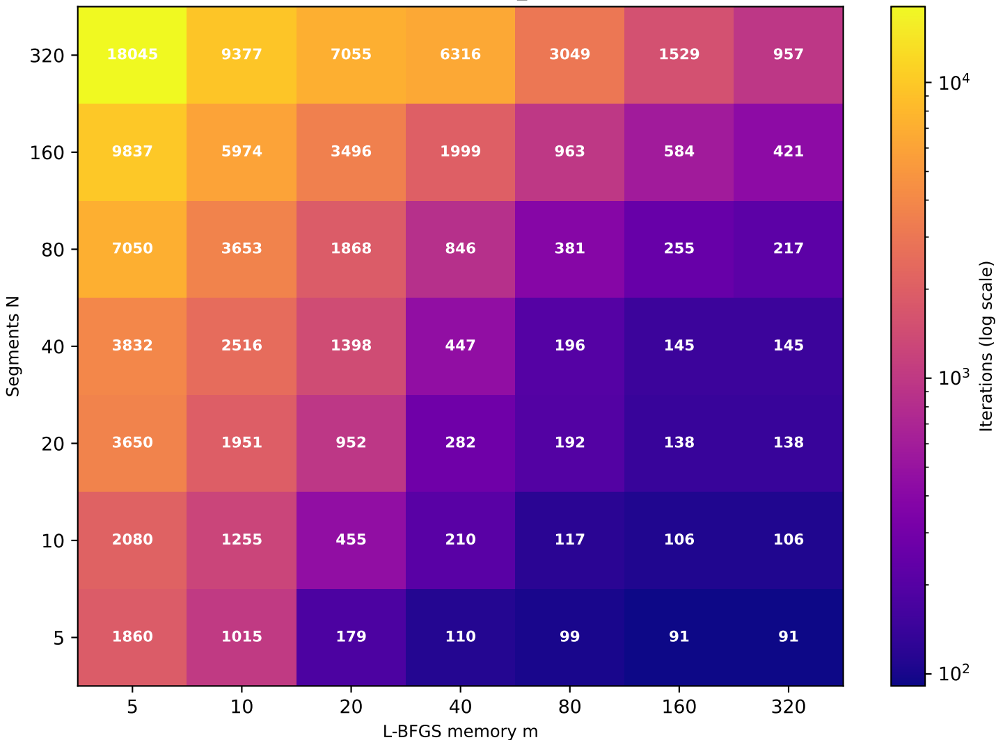
Recurrence T \approx 4.59 (target T=5 , rec_id=57) [49/49 converged]
